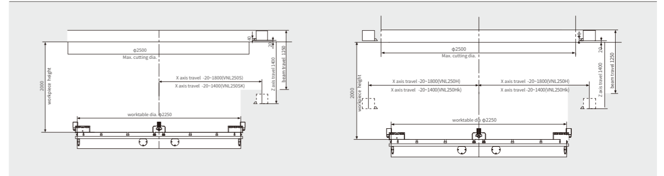
VNL250S/SK
