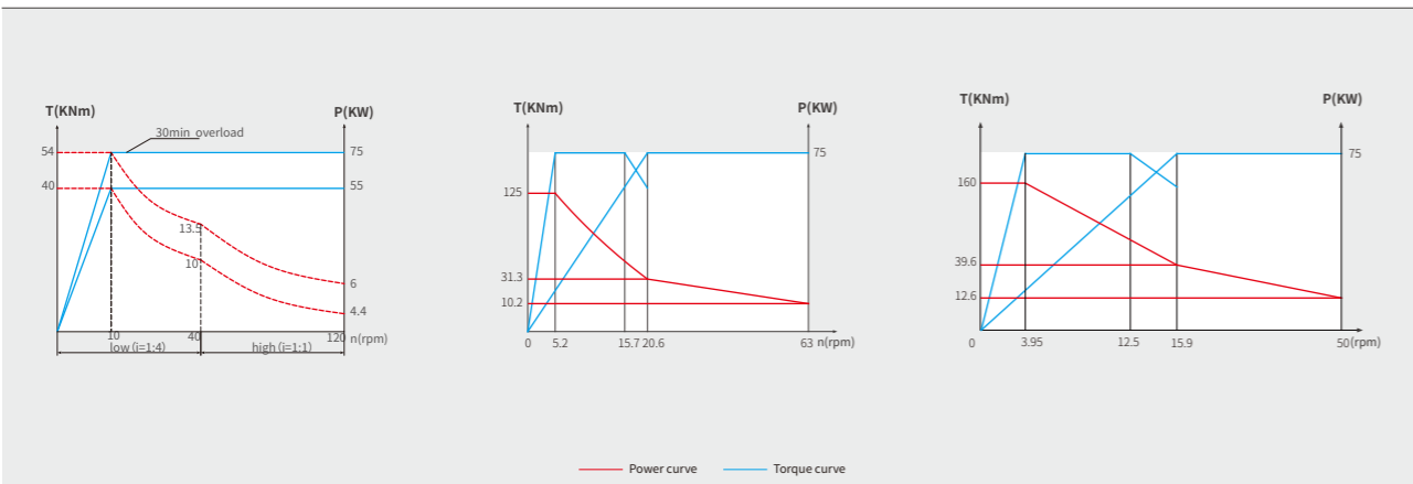
VNL250S/D/SK/DK/SF/DF/SFK/DFK
