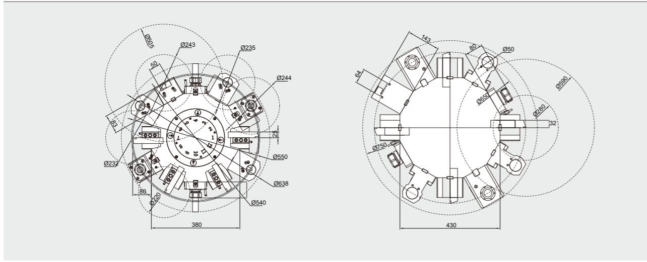
VNL40M/60M (BMT65)
