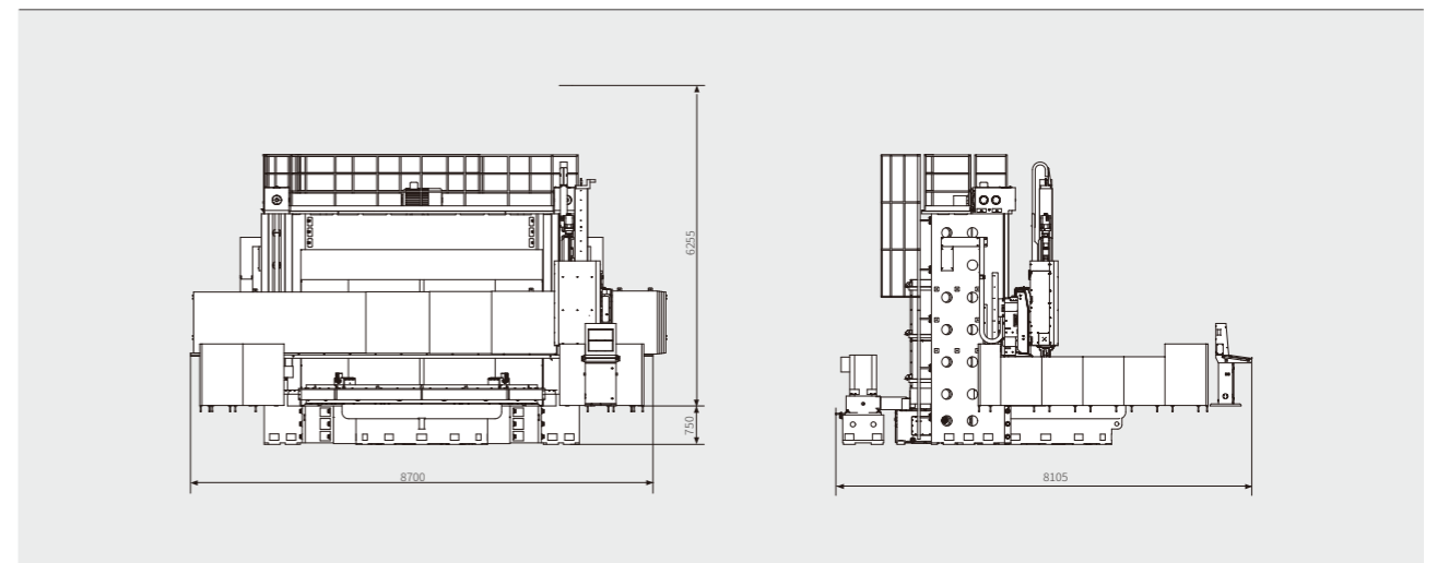
VNL500S/SK
