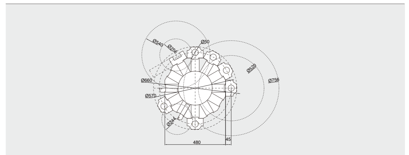
VNL100S/VNL100H
