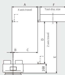
Horizontal 12-station Turret
