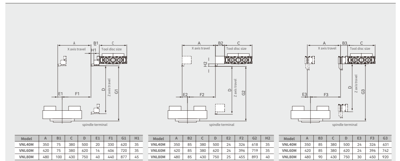
VNL40/60M/80M
