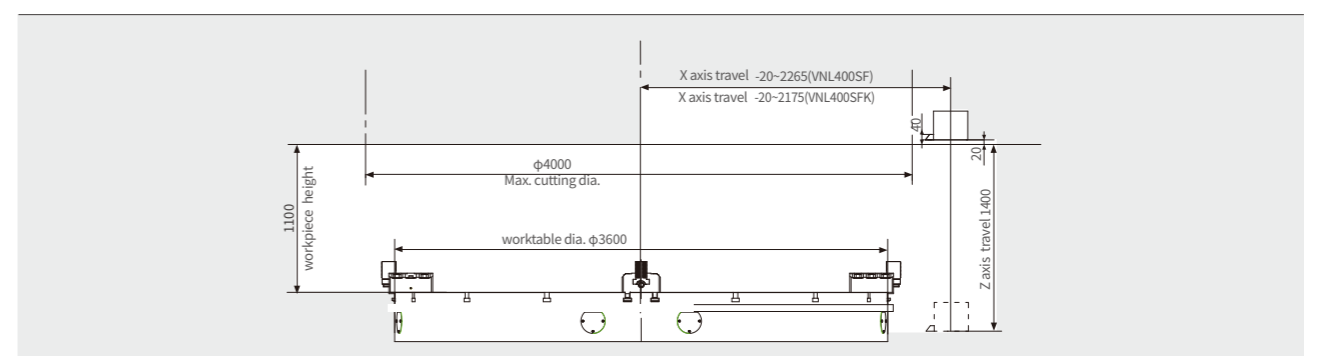
VNL400SF/SFK
