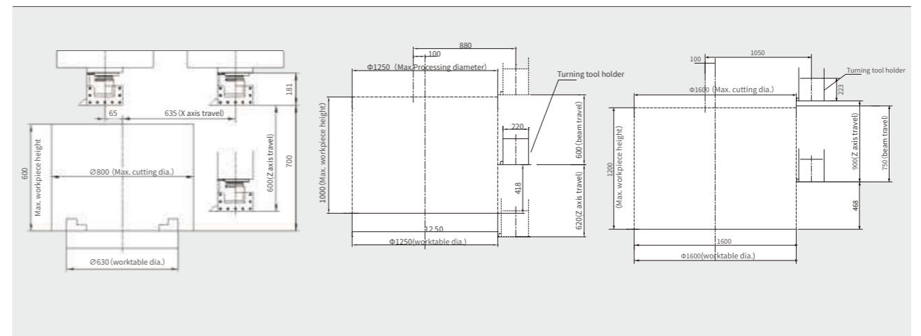
VNL80M
