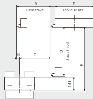
Horizontal 8-station Turret
