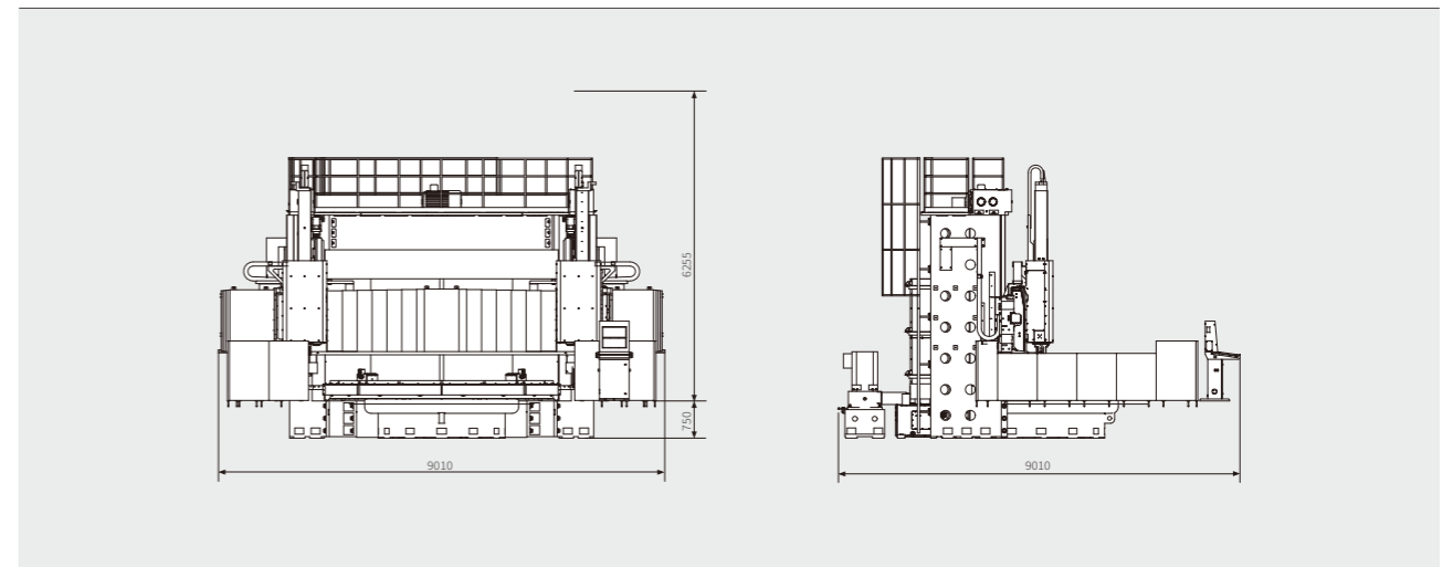
VNL500H/HK
