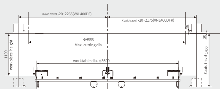
VNL400DF/DFK
